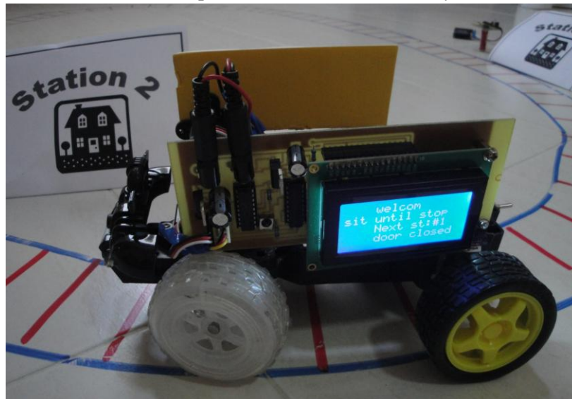
Figure 6. The assembled driverless train prototype
