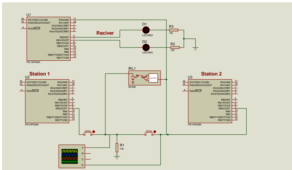
Figure 5. Schematic diagram showing the simulation of the IR sensors
