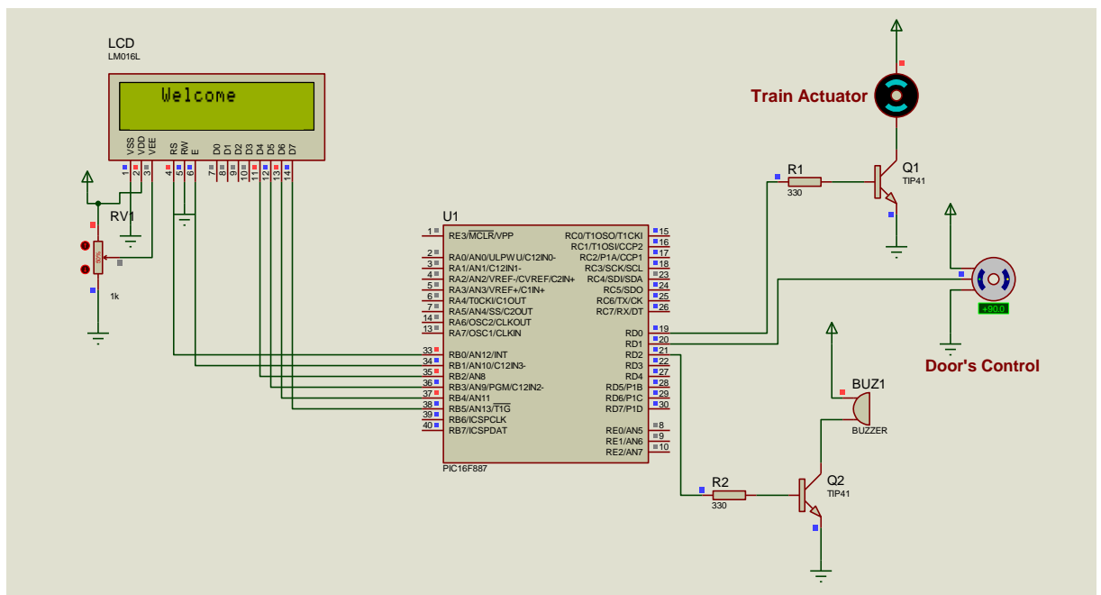
Figure 2. Schematic diagram showing the system simulation using Proteus software.
